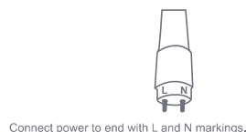
Diagram 2 – Connecting end
